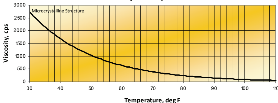
HB-230 Viscosity vs Temperature
