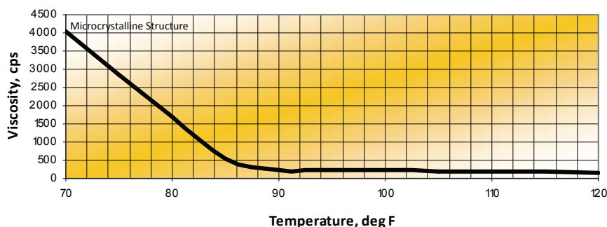
Honey Bee 230M Viscosity vs Temperature
